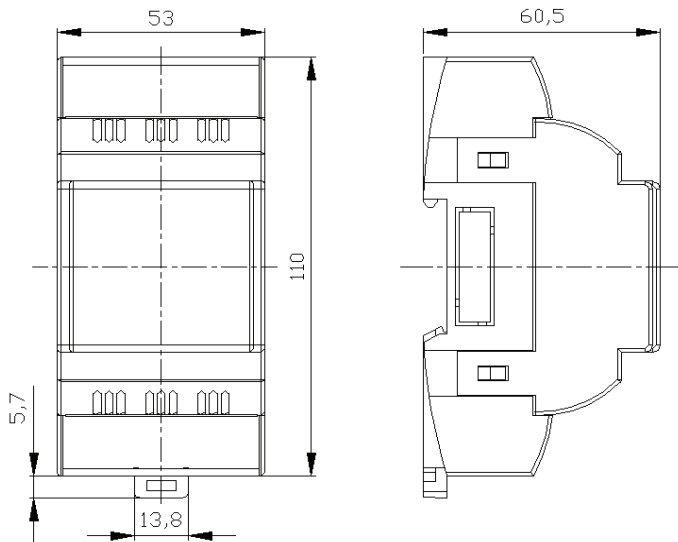
Figure 2. Meter dimensions
