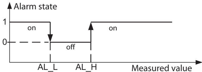
Figure 8. Alarm types
